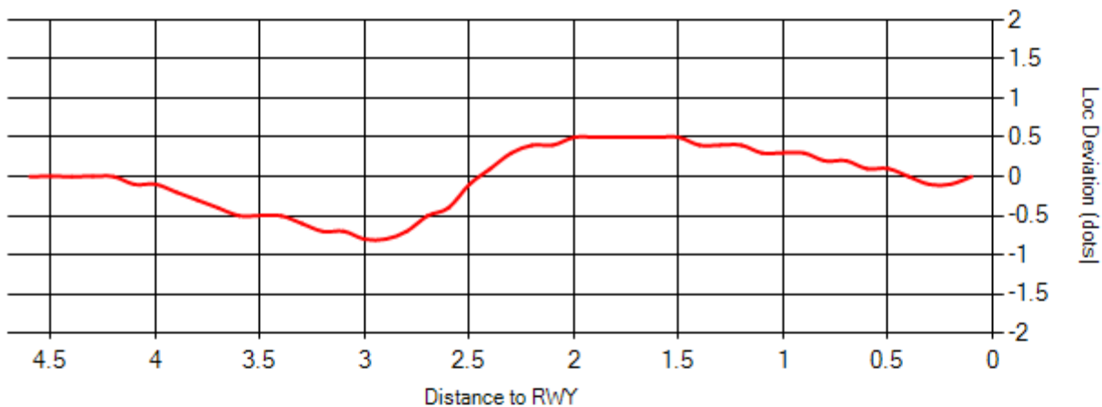
Localizer Deviation
