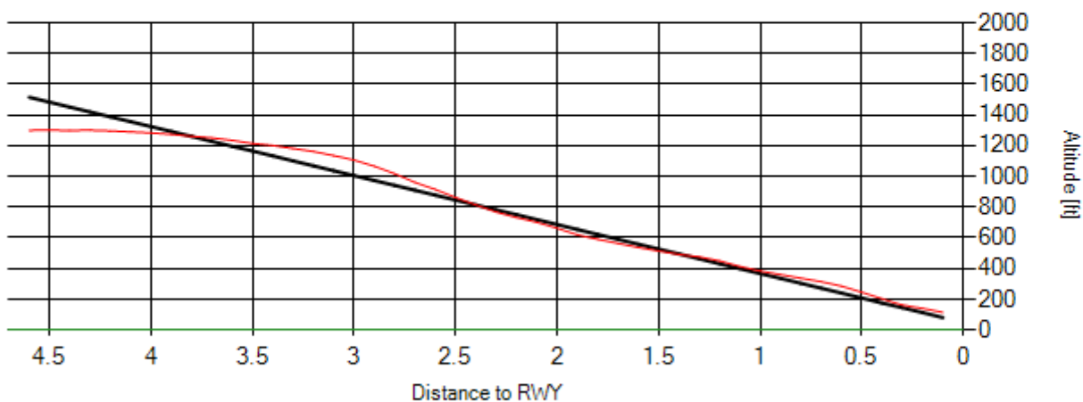
Glideslope Deviation
